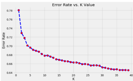
(b) Error Rate vs K value for Confirm v/s Recovered Cases
