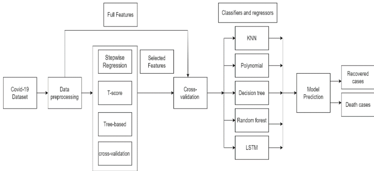
Figure 1: The Working of the Prediction Model Through a Flow Chart
