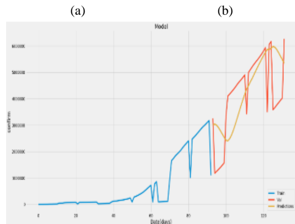
Figure 9 Prediction using LSTM Model (a) Date vs Confirmed Cases Graph using LSTM Model
